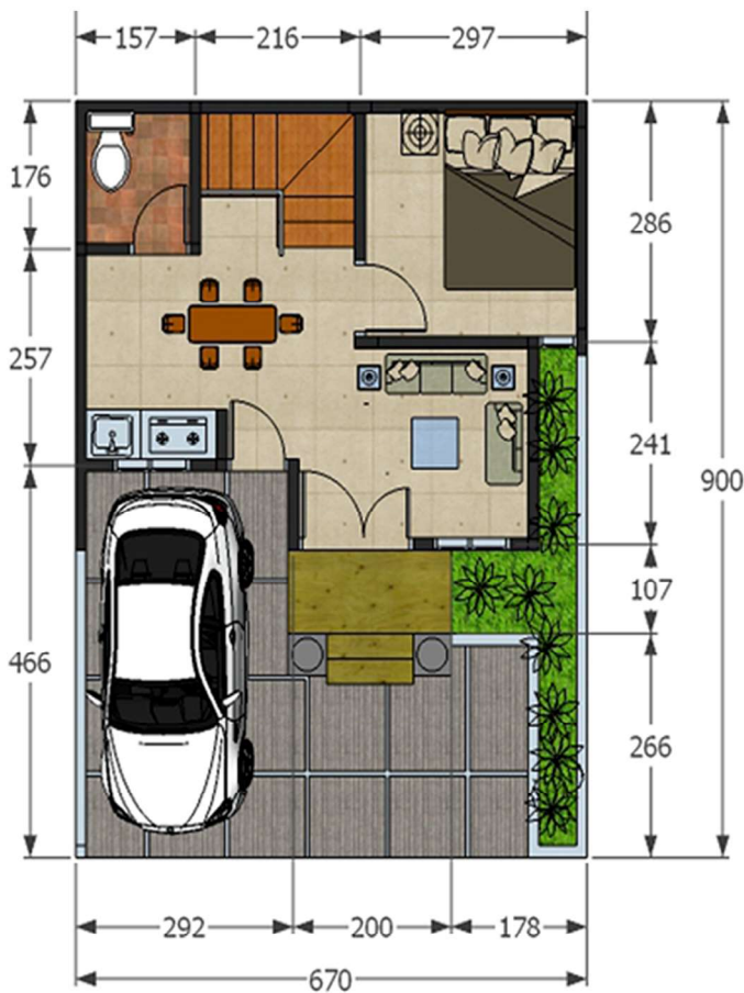
DENAH LANTAI.1
